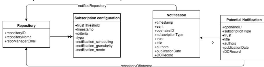
Figure 4 - Data model
