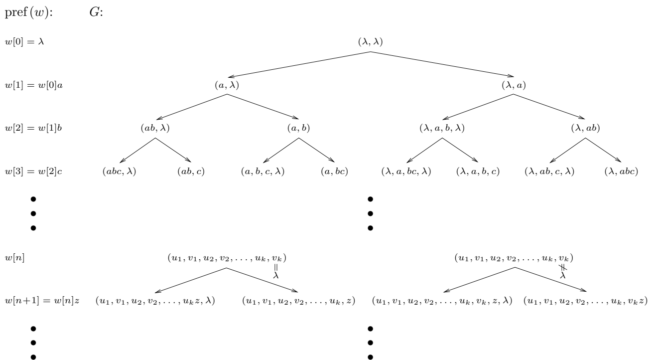
Fig. 1. Sketch of tree G = (\bigcup_{n \geq 0} V_n, E) .
