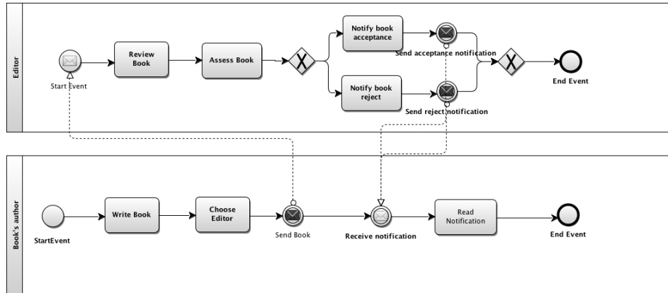
Figure 2. BPMN process diagram example 2
